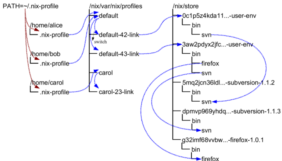
Figure 9.1: User environments
