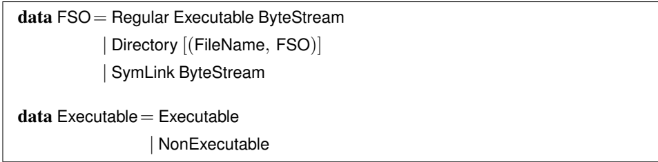
Figure 5.1.: Abstract syntax for file system objects
