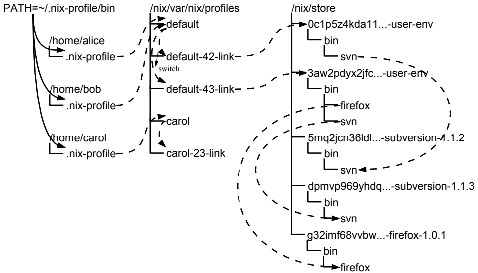
Figure 2.11.: User environments
